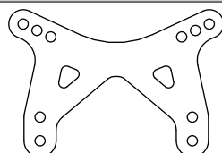
Carbon Front Shock Tower - Buggy 碳纤维前避震架-越野车 1pcs
